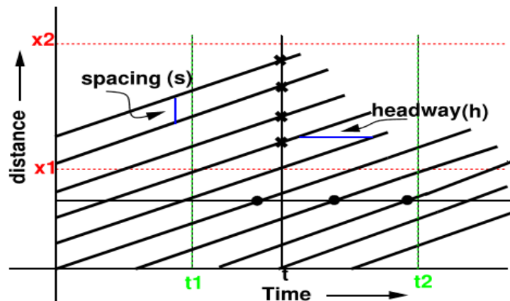
Fig. 12.2 Many vehicle
