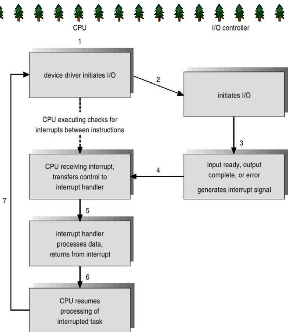
(Diagram of Interrupt-driven I/O cycle)
