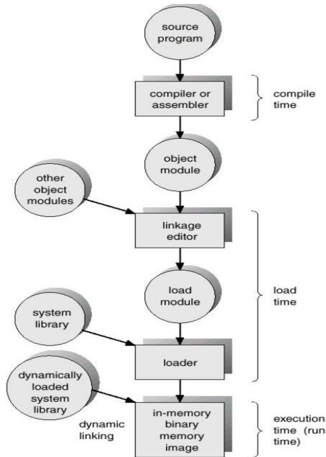
(Multistep processing of a user program.)
